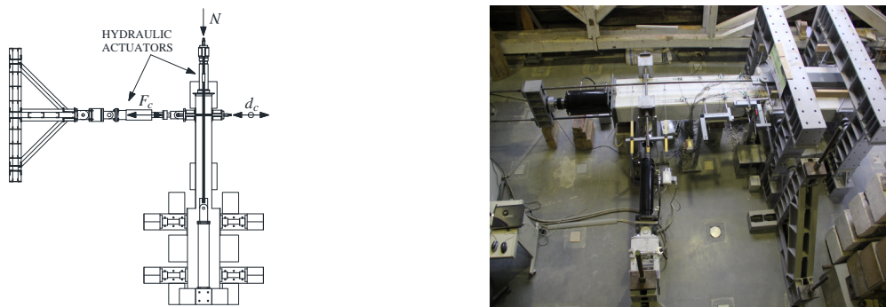
Figure 6. Test setup for column specimens.
