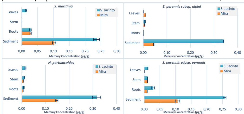
Figure 1: Mercury concentration (µg/g) in the sediment and different tissues (root, stem, and leaves) of the four species of halophyte plants, in the salt marshes of Mira and São Jacinto.
