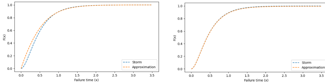
(a) OR(B, AND(C, OR(A, D))) with h=0.0050 .
