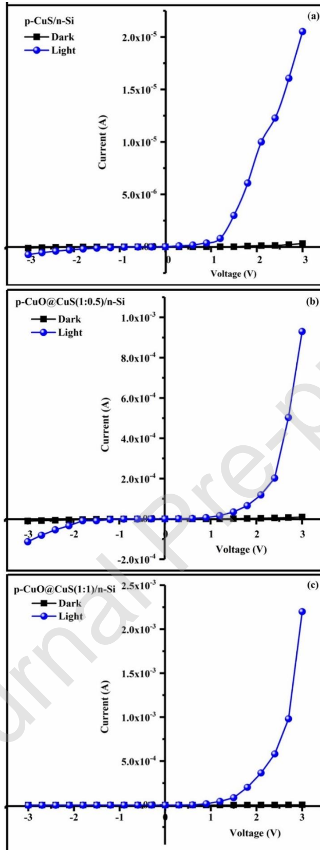
Figure 8 : I–V characteristics of (a) p-CuS/n-Si,(b) p-CuO@CuS/n-Si (1:0.5), (c) p-CuO@CuS/n-Si (1:1).
