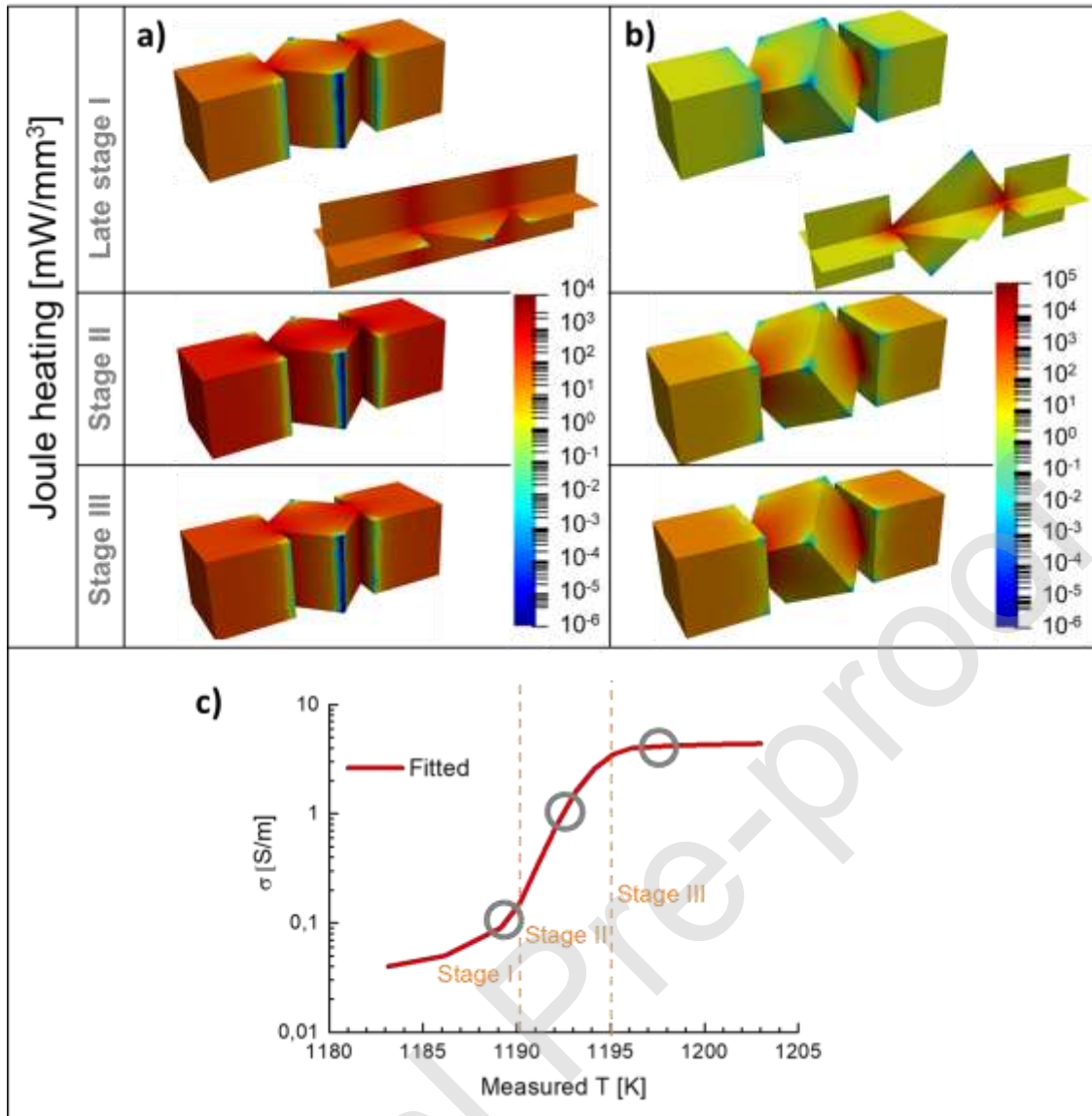
Figure 6 – Joule heating distribution (in mW/mm 3 ) for sharp contact arrangement of particles: (a) face/edge and (b) face/vertex. Three snapshots of the FLASH process are shown, corresponding to late stage I, stage II and stage III. A section view for late stage I case is also shown, for clarification. (c) represents the corresponding stages with the conductivity fitted curve overlaid with grey circles.
