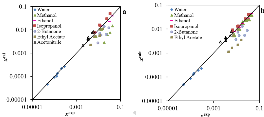
Figure 3: Comparison between experimental and calculated solubility for correlation: a) NRTL-SAC; b) NRTL-SAC + RSA.
