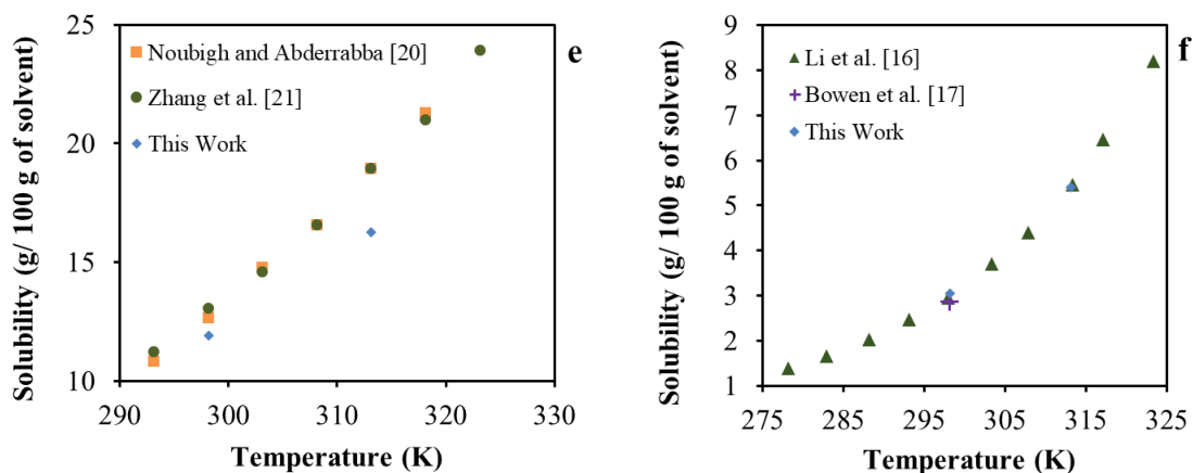
Figure 2: Comparison of the experimental solubility data obtained in this work with literature data [16,17,19–24]: (a) syringic acid + water; (b) vanillic acid + water; (c) veratric acid + water; (d) syringic acid + ethanol; (e) vanillic acid + ethanol; (f) veratric acid + ethanol.
