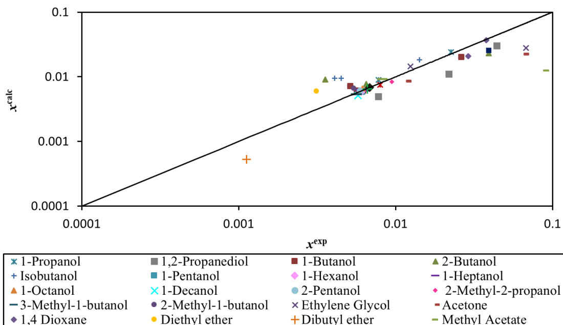
Figure 6: Comparison between experimental and calculated solubility data in the predicted set using the Abraham solvation model.
