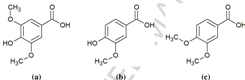
Figure 1: Chemical structures of: (a) syringic acid; (b) vanillic acid and (c) veratric acid.
