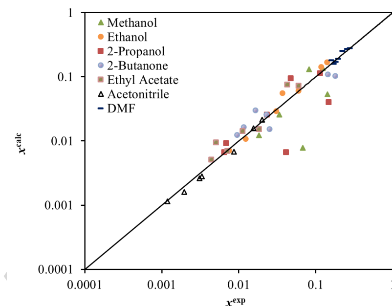
Figure 5: Comparison between experimental and calculated solubility in the organic solvents used in the estimation of the Abraham solute parameters.
