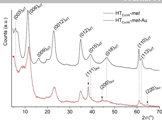
Figure 2. XRD powder patterns of \text{HT}_{\text{Co/Al-met}} and \text{HT}_{\text{Co/Al-met-Au}} . The peak at 2\theta = 5.74^\circ is due assigned to the 003 diffraction peak corresponding to the interlayer space containing the methionine guests. Diffraction peaks arising from \text{Au}_{\text{NP}} in \text{HT-met-Au} are highlighted with an arrow at 2\theta = 38.2^\circ , 44.4^\circ and 64.6^\circ . Diffraction patterns have been offset vertically for clarity.
