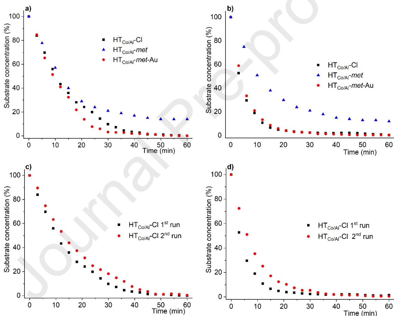
Figure 7. Time-dependent UV-Vis changes of rhodamine B (554 nm, a and c ) and rhodamine 6G (526 nm, b and d ) in the presence of the \text{HT}_{\text{Co/Al-Cl}} , \text{HT}_{\text{Co/Al-met}} and \text{HT}_{\text{Co/Al-met-Au}} catalysts. The plots in c and d show the kinetics for two consecutive catalytic reduction reactions of rhodamine B ( c ) and rhodamine 6G ( d ) in the presence of \text{HT}_{\text{Co/Al-Cl}} evidencing its little sensitivity to deactivation. Figure S7 shows the linearized plots of the reaction kinetics data.
