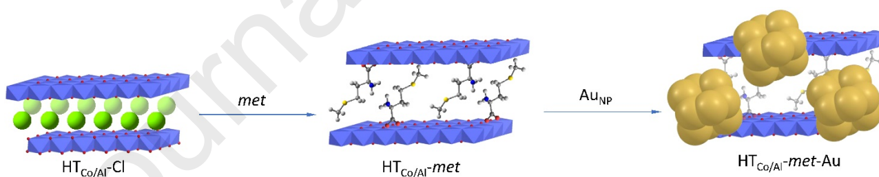
Scheme 1. Synthetic procedure for preparation of clay materials.
