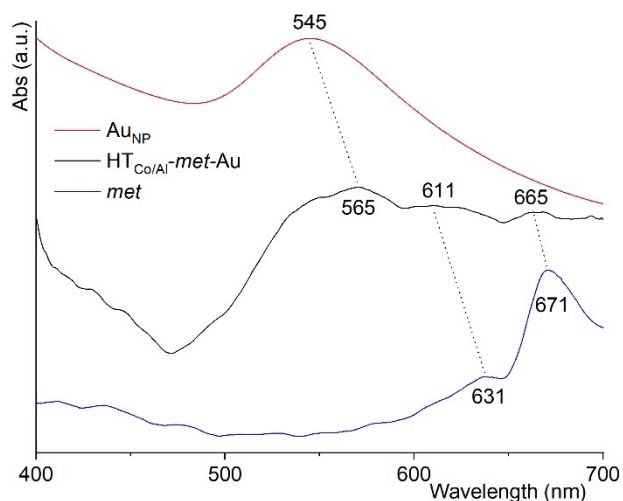
Figure 1. Electronic spectra of gold nanoparticles ( \text{Au}_{\text{NP}} ), methionine ( \text{met} ), and of the hybrid clay materials \text{HT}_{\text{Co/Al}}\text{-met-Au} and \text{HT}_{\text{Co/Al}}\text{-met} . The spectra of the hybrid materials were obtained as diffuse reflectance (DRUV) while the remaining were obtained from aqueous solutions in transmission mode. Spectra have been offset vertically for clarity.
