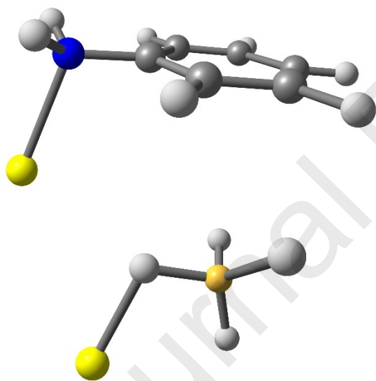
Figure 6. DFT optimized structures of Au(0) complexes with aniline (top) and borohydride anion (bottom).
