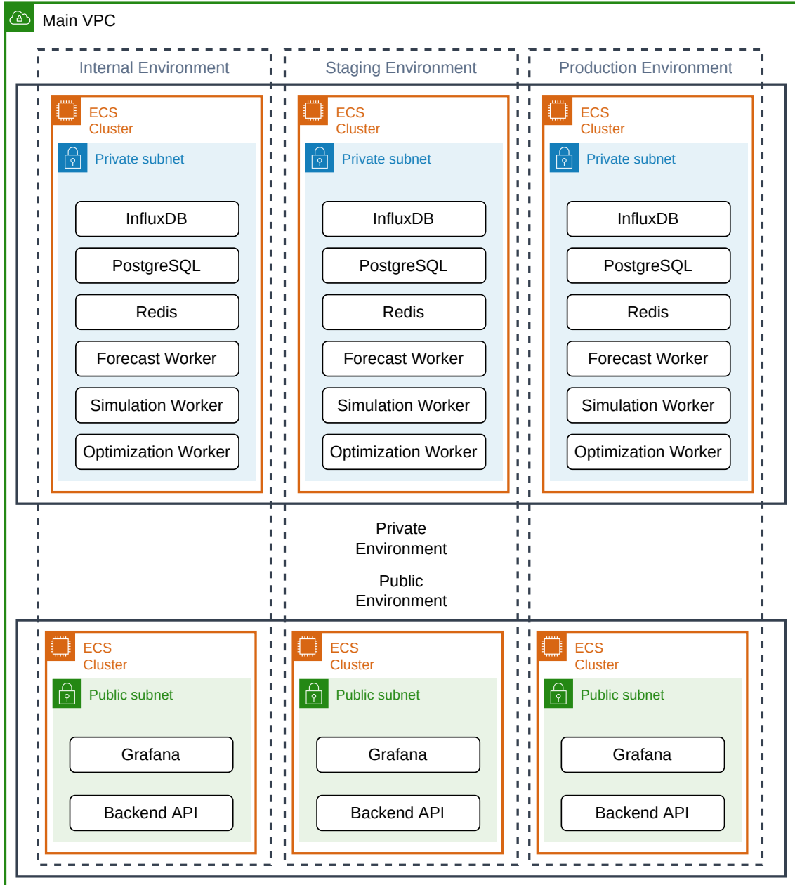
Figure 3.12: The VPC is divided in six different ECS Clusters, each with their subnet. The VPC is divided in two ways between Public and Private Environments and also divided in three parts, one for Internal use and the other two for Staging and Production Environments, respectively.
