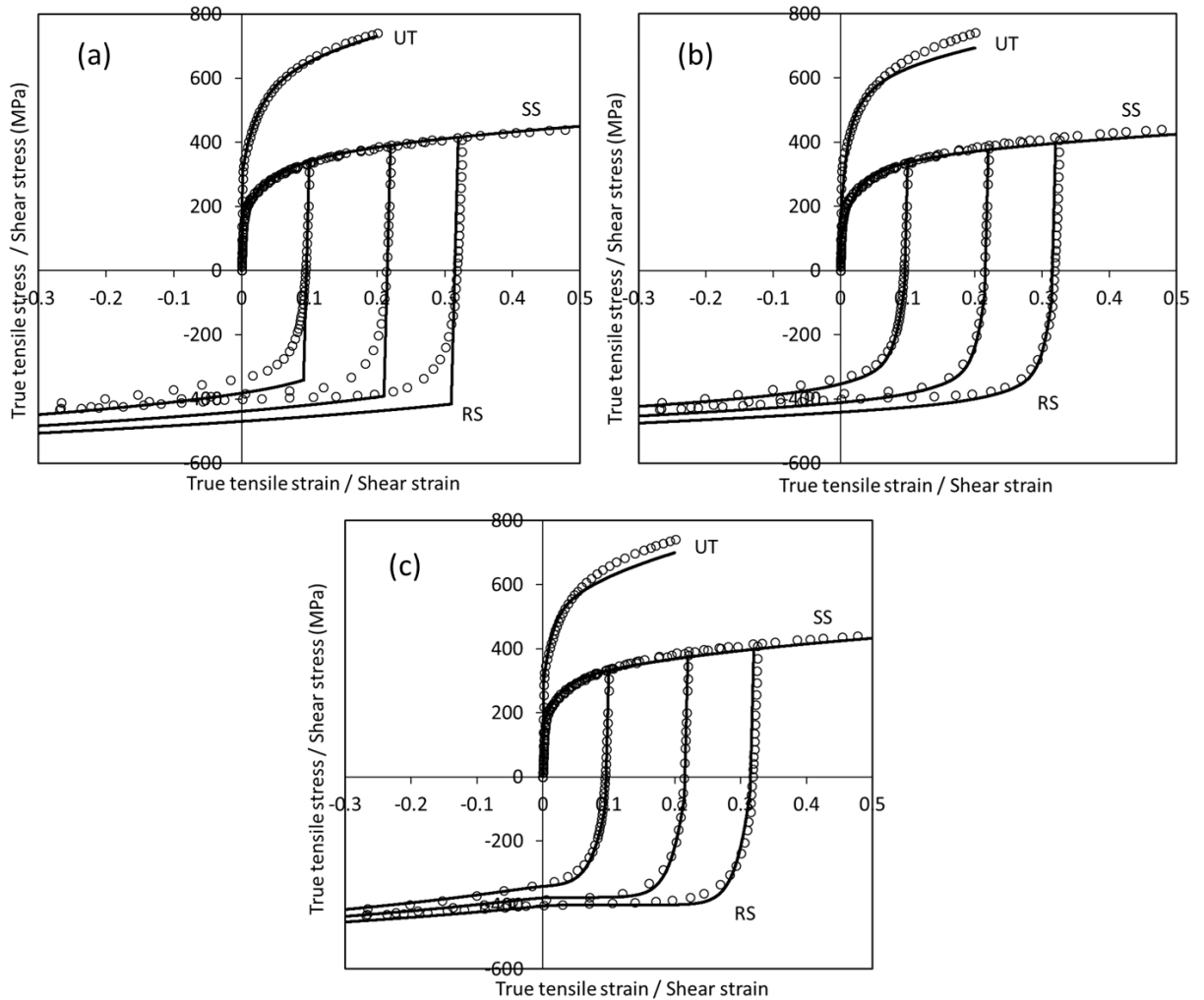
Fig. 2. Rheological predictions (solid line) of classical type hardening models: (a) Isotropic; (b) Combined; (c) Microstructural, and their comparisons of experimental results (symbols).
