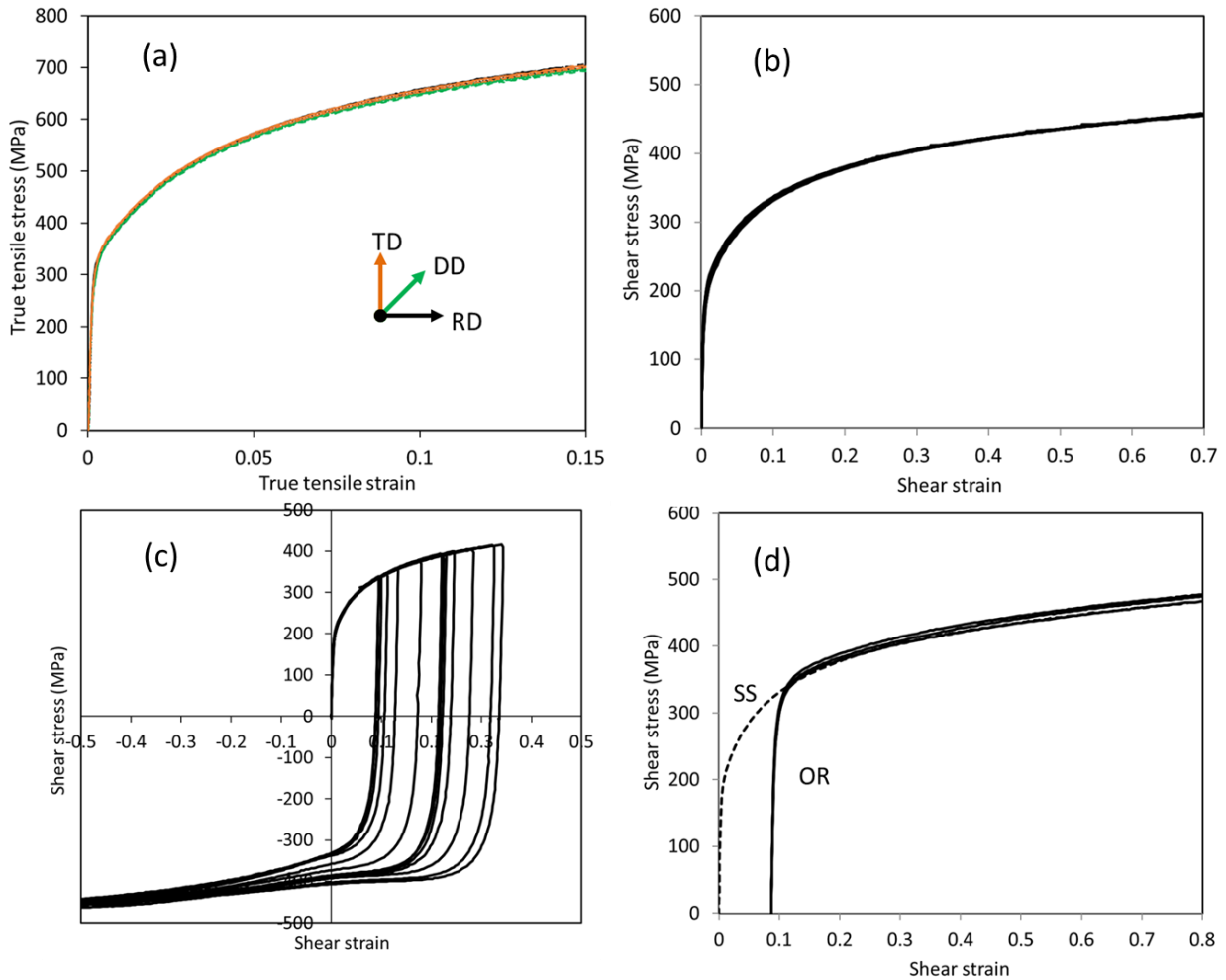
Fig. 1. Material characterization results of DP600: (a) uniaxial tension (UT) in RD (black curves), DD (green curves) and TD (orange curves); (b) simple shear (SS) in RD; (c) reverse shear (RS) in RD; (d) uniaxial 5% tensile pre-strain followed by simple shear (OR) in RD. For graphical convenience only, the tensile pre-strain was converted here into shear pre-strain using the von Mises assumption.
