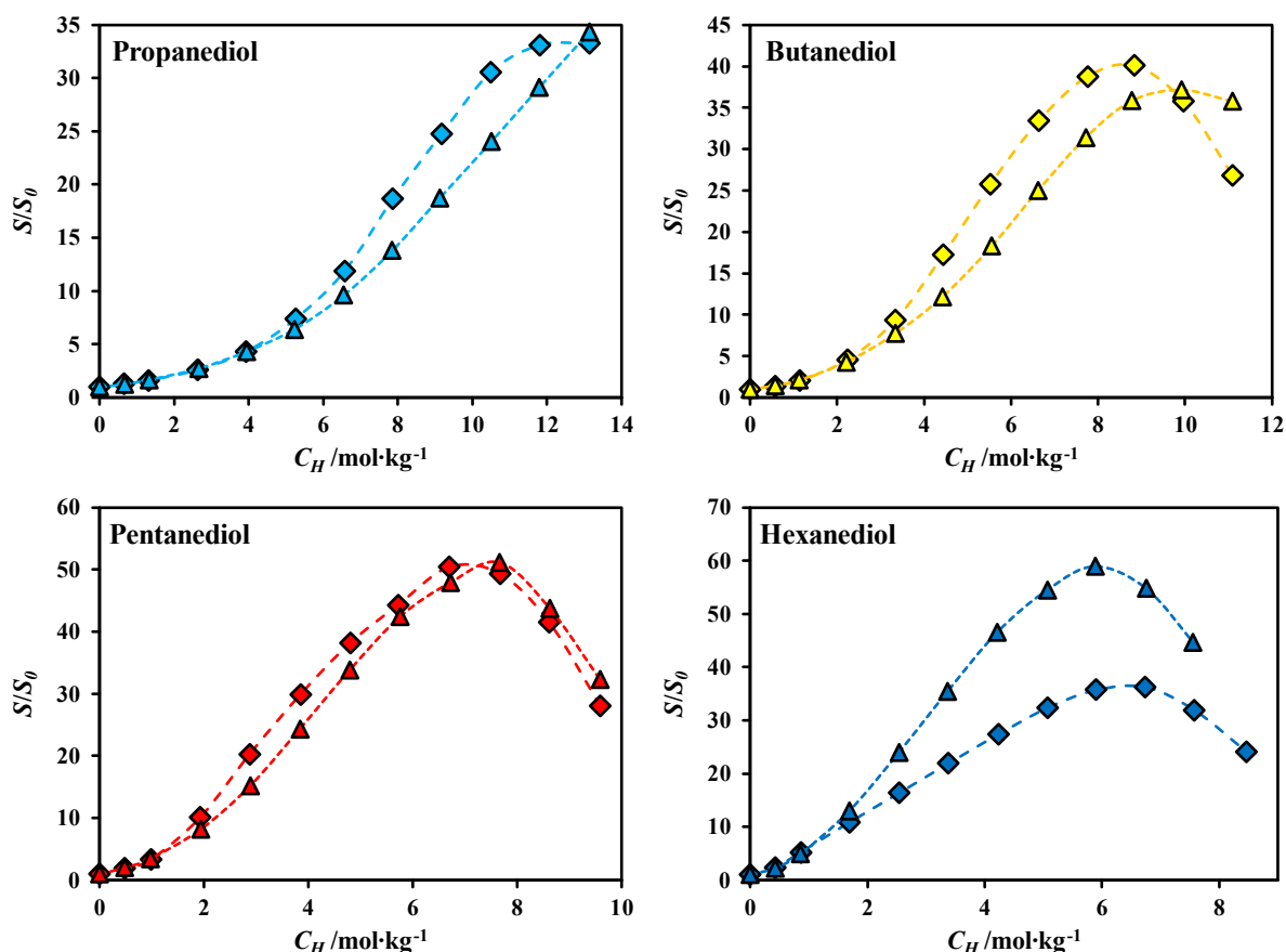
Figure 3. Solubility enhancement of syringic acid in aqueous solutions of propanediol (1,2-propanediol ♦ and 1,3-propanediol ▲), butanediol (1,2-butanediol ♦ and 1,4-butanediol ▲), pentanediol (1,2-pentanediol ♦ and 1,5-pentanediol ▲), and hexanediol (1,2-hexanediol ♦ and 1,6-hexanediol ▲), as a function of hydrotrope concentration, at 303.2 K. S/S_0 is the relative solubility of the solute and C_H is the concentration of hydrotrope per kg of solution (solute-free basis). Dashed lines are visual guides.
