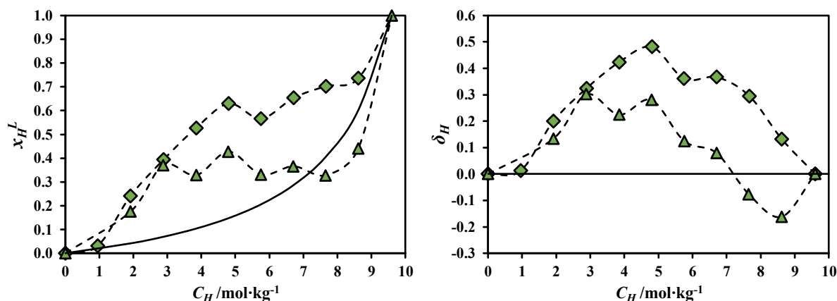
Figure 9. Local composition of hydrotrope around the pyrene probe (left) and difference between local and bulk compositions (right) for aqueous solutions of 1,2-pentanediol (◆) or 1,5-pentanediol (▲). C_H is the concentration of hydrotrope per kg of solution (solute-free basis). Dashed lines are visual guides and full lines represent thermodynamic ideality (local composition equal to bulk composition).
