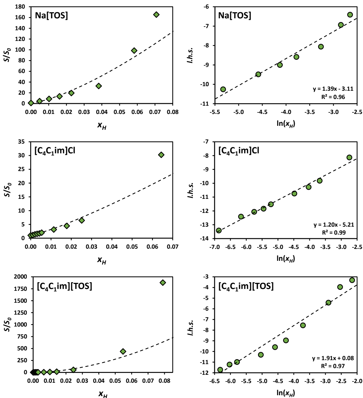
Figure S6. Left: solubility enhancement ( S/S_0 ) of ibuprofen in aqueous solutions of ionic hydrotropes ( \blacklozenge ) along with the fitted curve (dashed line) obtained using the cooperative hydrotropy model. Right: the linearized form of the cooperative hydrotropy model for each hydrotropic system, where the vertical axis is the left-hand side of Equation S1 and the dashed line is the straight line obtained using the method of least squares. Data measured in this work or taken from the literature. 5
