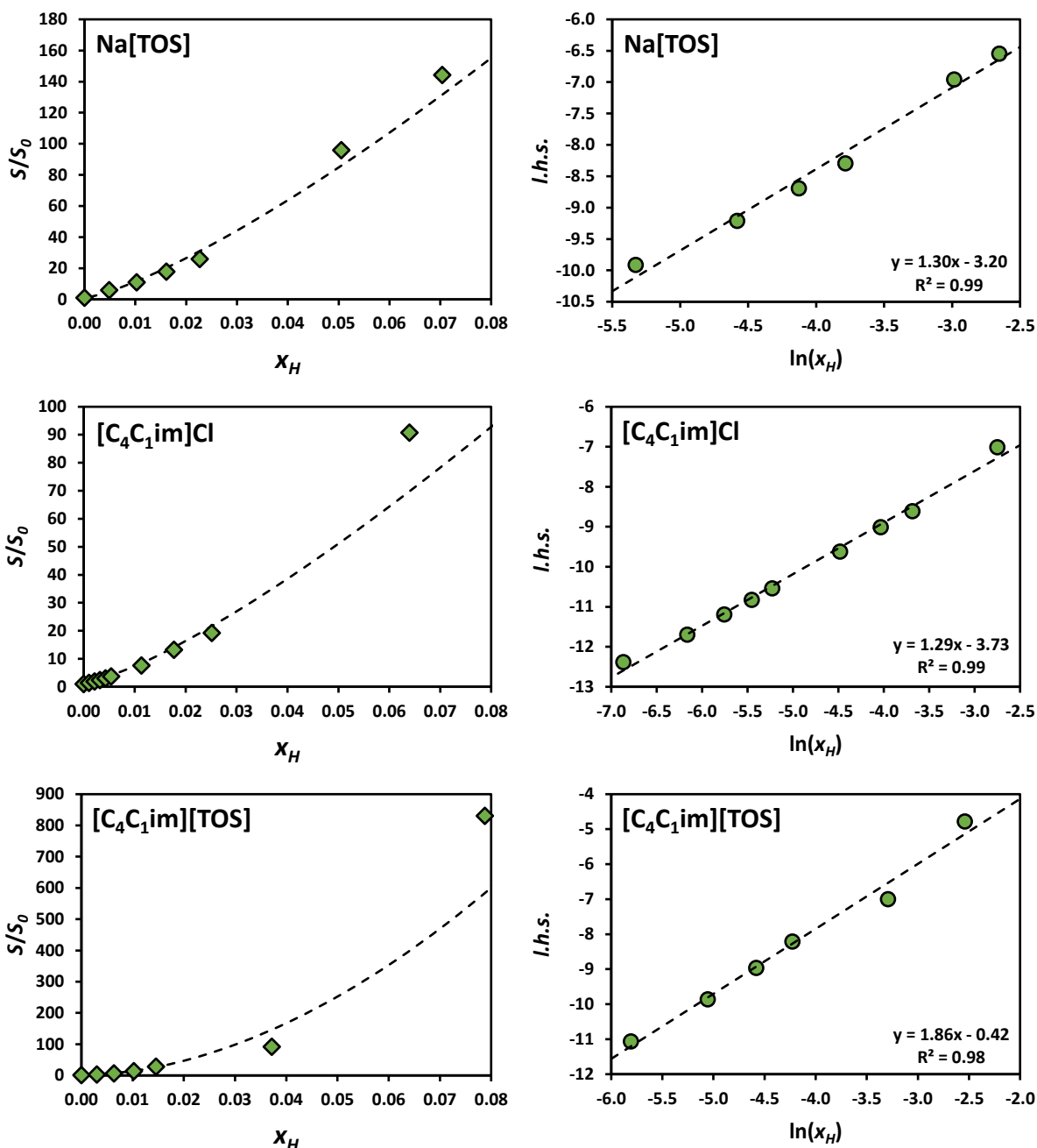
Figure S5. Left: solubility enhancement ( S/S_0 ) of naproxen in aqueous solutions of ionic hydrotropes ( \blacklozenge ) along with the fitted curve (dashed line) obtained using the cooperative hydrotropy model. Right: the linearized form of the cooperative hydrotropy model for each hydrotropic system, where the vertical axis is the left-hand side of Equation S1 and the dashed line is the straight line obtained using the method of least squares.
