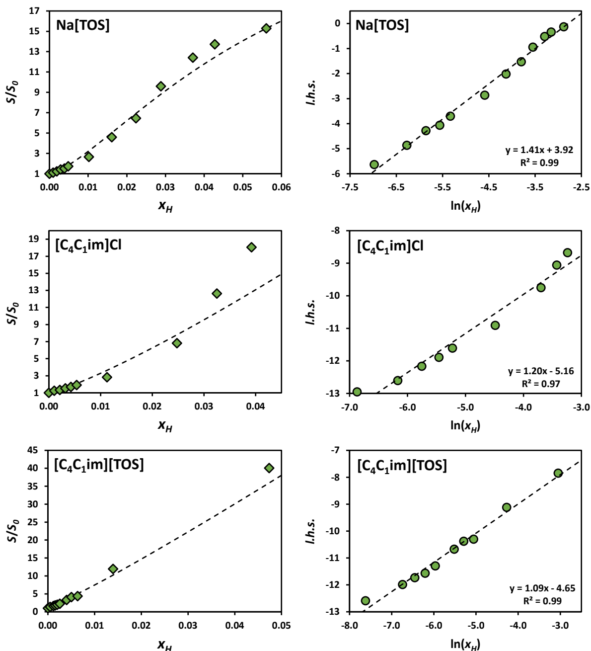
Figure S3. Left: solubility enhancement ( S/S_0 ) of vanillin in aqueous solutions of ionic hydrotropes ( \diamond ) along with the fitted curve (dashed line) obtained using the cooperative hydrotropy model. Right: the linearized form of the cooperative hydrotropy model for each hydrotropic system, where the vertical axis is the left-hand side of Equation S1 and the dashed line is the straight line obtained using the method of least squares. Data measured in this work or taken from the literature. 4
