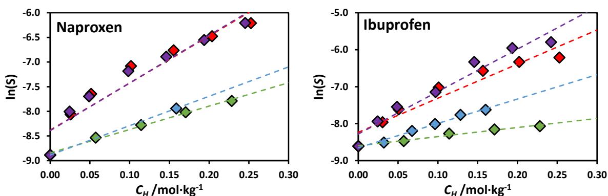
Figure S8. Aqueous solubility enhancement ( S/S_0 ) of naproxen and ibuprofen as a function of the molal concentration (solute-free basis) of [C_4C_1im]Cl ( \blacklozenge ), [C_4C_1im][TOS] ( \blacklozenge ), [C_4C_1im][SCN] ( \blacklozenge ), or [C_4C_1im][DCA] ( \blacklozenge ), at 303.2 K, in the narrow composition range 0-0.3 mol·kg -1 . The dashed lines are the straight line obtained using the method of least squares.
