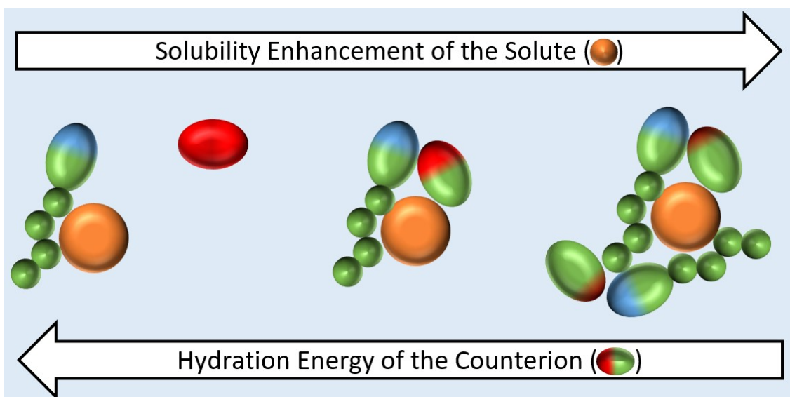
Figure S10. Schematic illustration of the behaviour of the counterion as its Gibbs hydration energy decreases. In the first case the counterion interacts too extensively with water and does not minimize the charge of the hydrotrope-solute cluster, corresponding to the commonly used small, densely charged counterions such as sodium or chloride. In the second and third cases, the counterion is progressively less hydrated and, thus, more available to move into the vicinity of the solute-hydrotrope cluster, minimizing charge repulsion between hydrotrope ions and leading to larger and more stable clusters.
