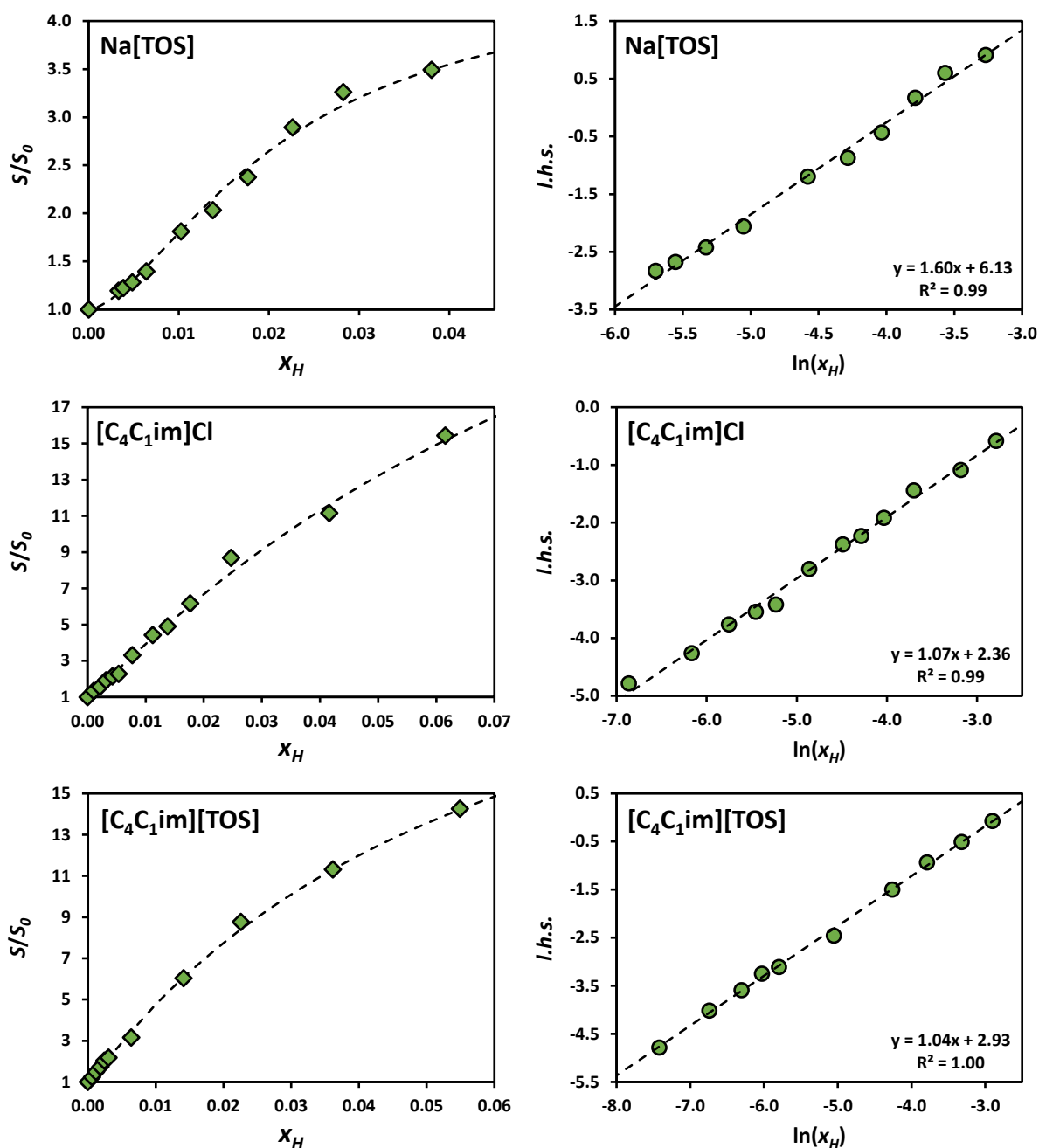
Figure S2. Left: solubility enhancement ( S/S_0 ) of gallic acid in aqueous solutions of ionic hydrotropes ( \blacklozenge ) along with the fitted curve (dashed line) obtained using the cooperative hydrotropy model. Right: the linearized form of the cooperative hydrotropy model for each hydrotropic system, where the vertical axis is the left-hand side of Equation S1 and the dashed line is the straight line obtained using the method of least squares. Data measured in this work or taken from the literature. 4
