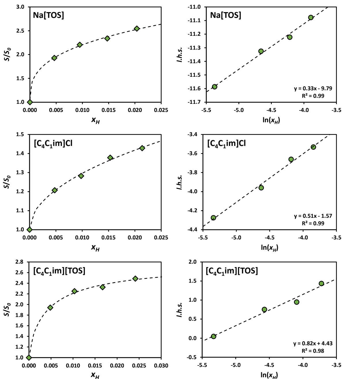
Figure S1. Left: solubility enhancement ( S/S_0 ) of caffeine in aqueous solutions of ionic hydrotropes ( \blacklozenge ) along with the fitted curve (dashed line) obtained using the cooperative hydrotropy model. Right: the linearized form of the cooperative hydrotropy model for each hydrotropic system, where the vertical axis is the left-hand side of Equation S1 and the dashed line is the straight line obtained using the method of least squares.
