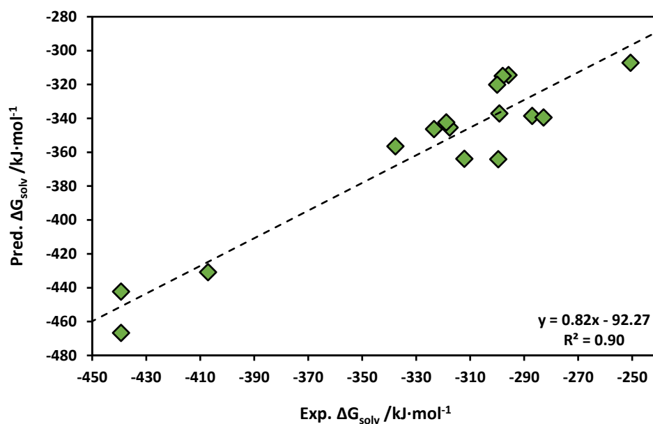
Figure S9. Correlation between the experimental Gibbs energy of solvation ( \text{Exp. } \Delta G_{\text{solv}} ) 11 and the Gibbs energy of solvation ( \text{Pred. } \Delta G_{\text{solv}} ) estimated using COSMO-RS of several anions at 298.2 K in water.
