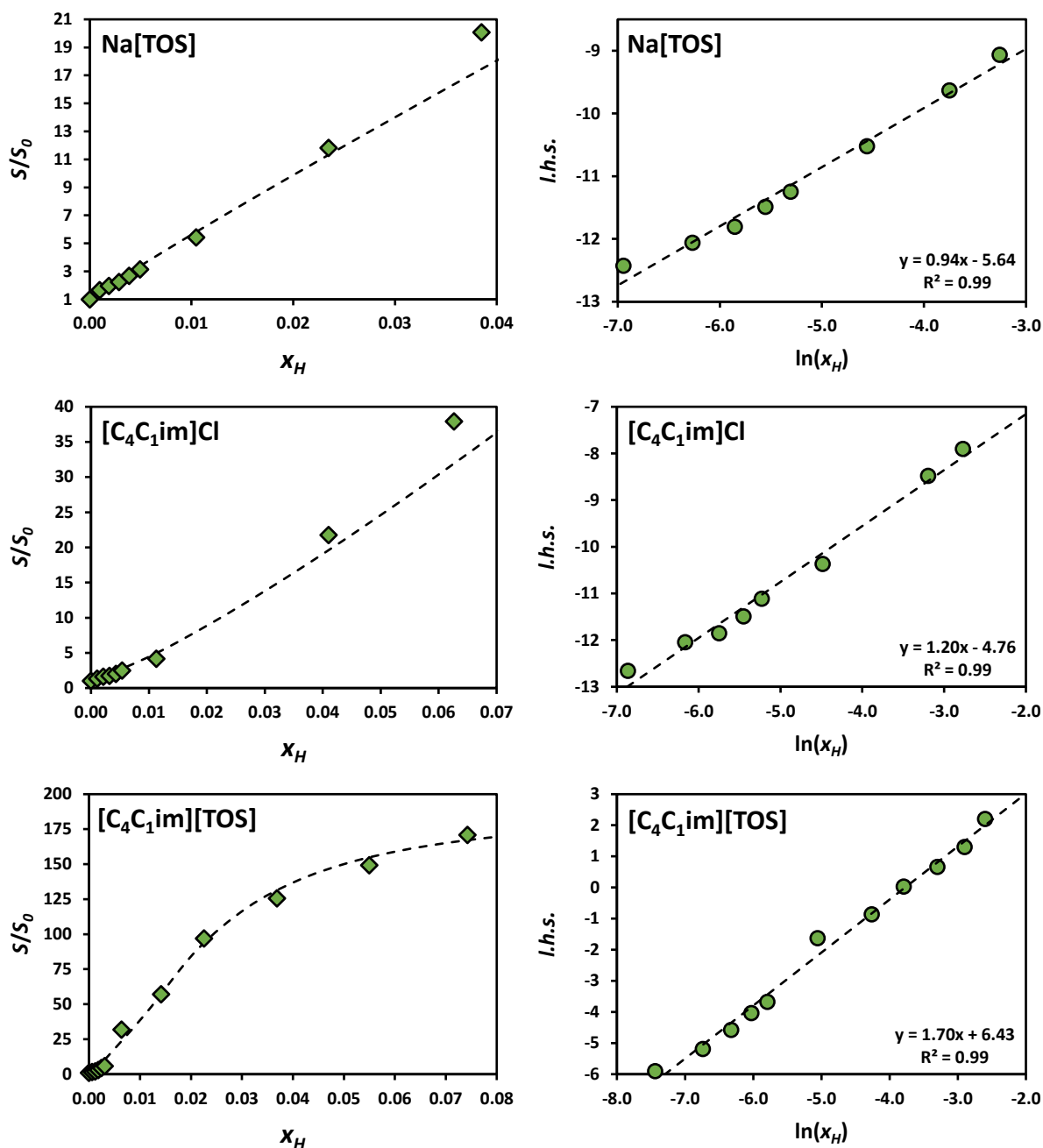
Figure S4. Left: solubility enhancement ( S/S_0 ) of syringic acid in aqueous solutions of ionic hydrotropes ( \blacklozenge ) along with the fitted curve (dashed line) obtained using the cooperative hydrotropy model. Right: the linearized form of the cooperative hydrotropy model for each hydrotropic system, where the vertical axis is the left-hand side of Equation S1 and the dashed line is the straight line obtained using the method of least squares.
