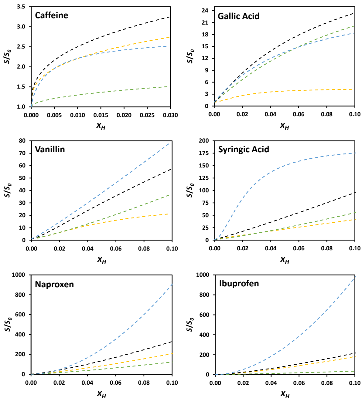
Figure S7. Solubility curves of the studied solutes in aqueous Na[TOS] (- - -), [C 4 C 1 im]Cl (- - -), and [C 4 C 1 im][TOS] (- - -), obtained using the cooperative hydrotropy model, and sum of the solubility curves of the solutes in Na[TOS] and [C 4 C 1 im]Cl (- - -), obtained using Equation S4.
