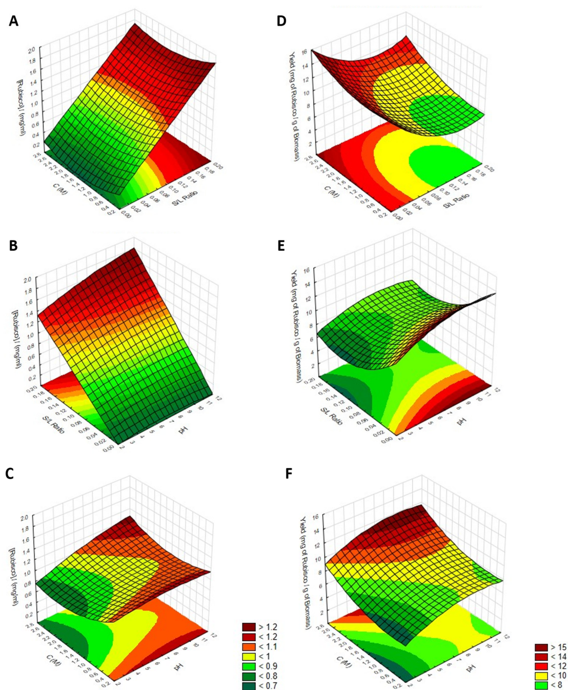
Figure 5. Response surfaces corresponding to the concentration of extracted RuBisCO (left) and yield of extraction (right) with the following combined parameters: (A,D) [Ch]Cl concentration and solid-liquid ratio; (B,E) solid-liquid ratio and pH; and (C,F) [Ch]Cl concentration and pH.
