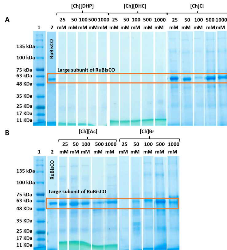
Figure 3. SDS-PAGE loaded and run on a polyacrylamide gel (stacking: 4% and resolving: 20%) stained with BlueSafe. Effect of IL concentration in the RuBisCO's extraction from spinach using the following experimental conditions: IL concentration of 25 mM–1000 mM, 600 rpm, 0.10 solid-liquid ratio, solid-liquid extraction during 30 min at 29 °C. Lanes 1, Gel (A,B): Standard molecular weights; Lanes 2, Gel A and B: 1 mg/mL of commercial RuBisCO dissolved in PBS.
