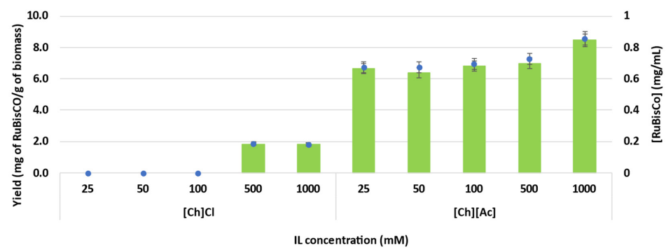
Figure 4. RuBisCO's extracted concentration (mg/mL) (blue symbols) and yield (green bars) after extraction from spinach leaves using different concentrations of IL (25 mM, 50 mM, 100 mM, 500 mM and 1 M), a solid-liquid ratio of 0.10 in a solid-liquid extraction, 600 rpm for 30 min at 29 °C.
