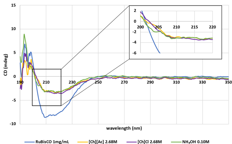
Figure 8. CD spectrums of the standard solution of RuBisCO, of the extracts with IL aqueous solutions at optimal conditions and of the extract with \text{NH}_4\text{OH} aqueous solution.
