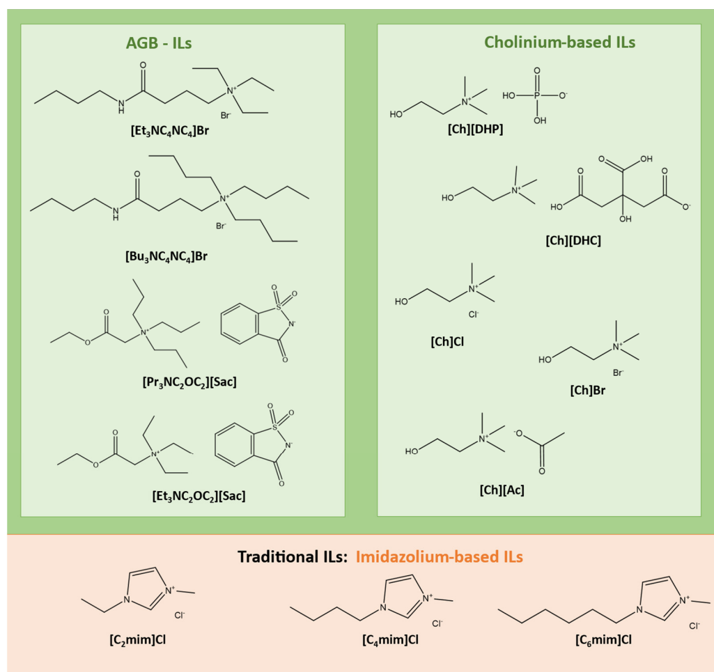
Figure 1. Structures and abbreviations of the ILs used in this work.
