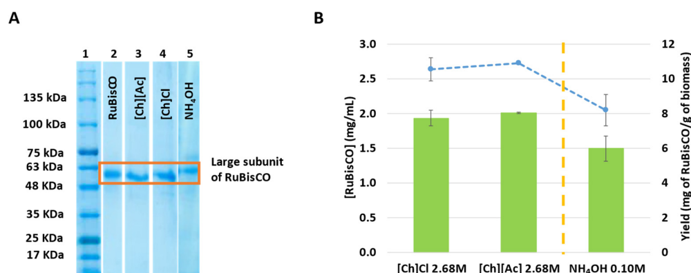
Figure 7. (A) SDS-PAGE loaded and run on a polyacrylamide gel (stacking: 4% and resolving: 20%) stained with BlueSafe. Lane 1: Standard molecular weights; Lane 2: 1 mg/mL commercial RuBisCO. (B) RuBisCO's yield (blue symbols and bar) and RuBisCO's concentration (green bars). The extractions were executed at the optimal conditions for both ILs and with a solution of \text{NH}_4\text{OH} of 0.10 M at pH 11. The agitation, time of extraction and temperature were maintained (600 rpm, 30 min, at 29^\circ\text{C} ).
