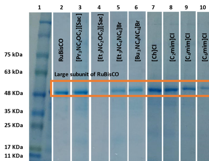
Figure 2. SDS-PAGE loaded on a polyacrylamide gel (stacking: 4% and resolving: 20%) stained with BlueSafe. Effect of IL aqueous solutions in the RuBisCO's extraction from spinach using the following experimental conditions: IL concentration of 3.3 mM, 0.10 solid-liquid ratio, solid-liquid extraction time 30 min at 29 °C. Lane 1: Standard molecular weights; Lane 2: 1 mg/mL commercial RuBisCO.
