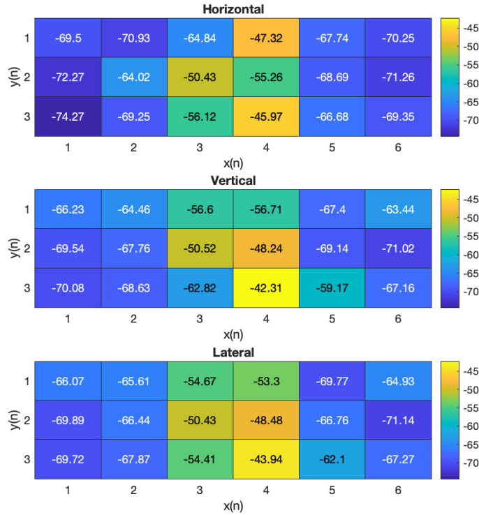
Figure 7.2: RSSI reading results for the different considered tag orientations in dBm
