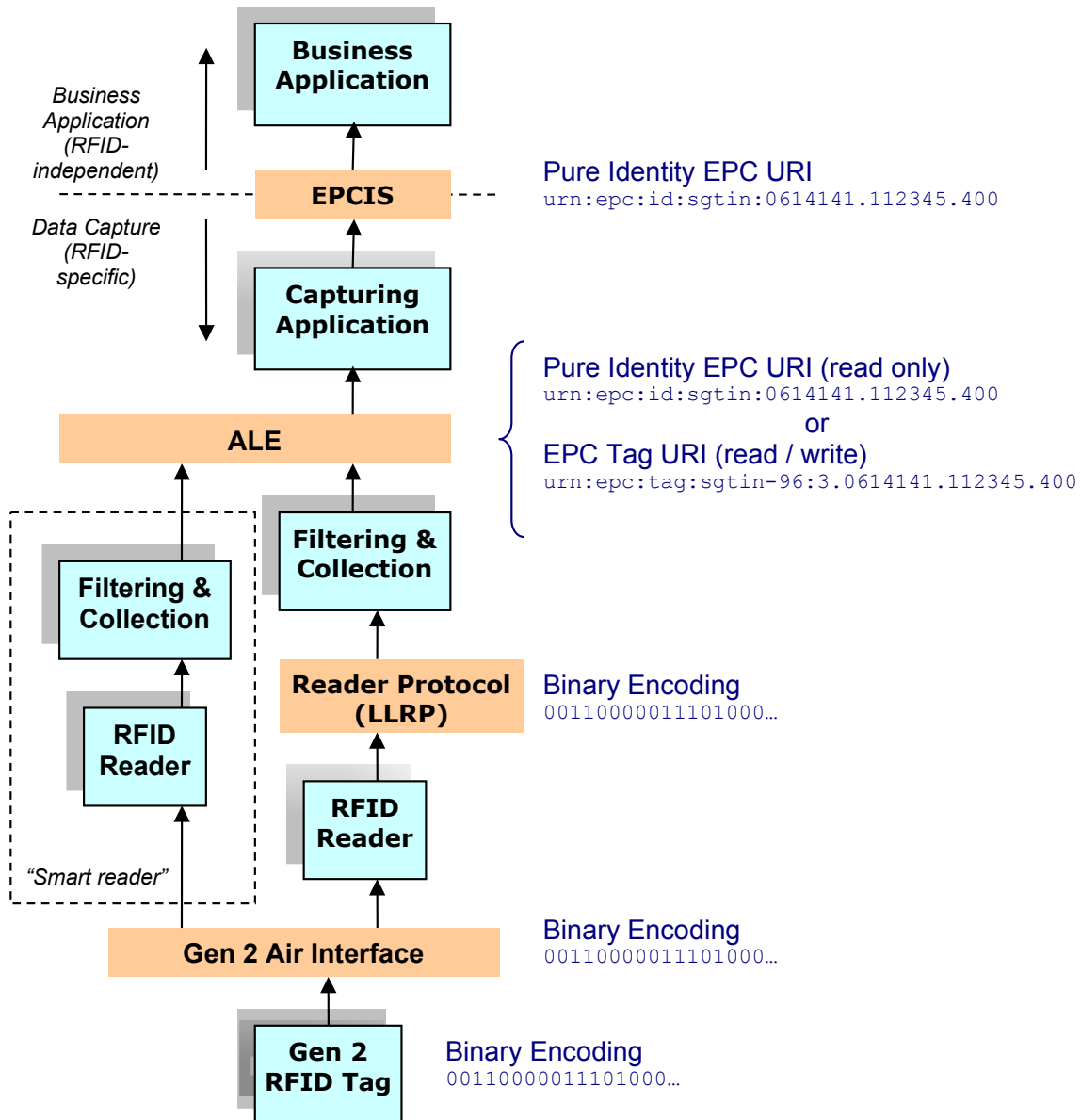
Figure 3.1: EPCGlobal Architecture Framework baseline example with EPC representations used at each level [52]
