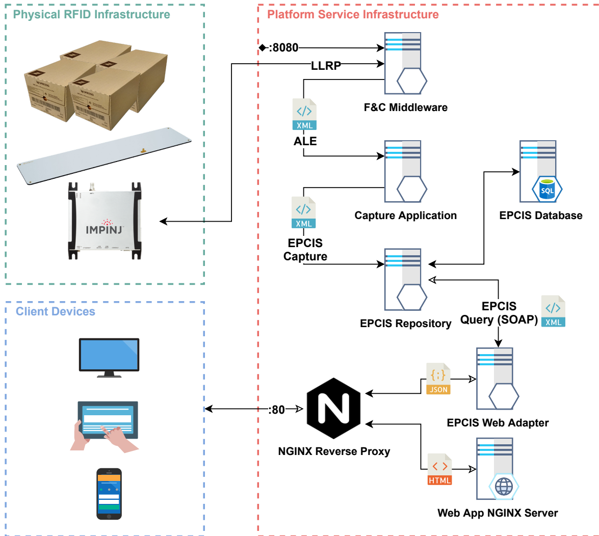
Figure 6.1: Overview of the solution architecture developed in this dissertation
