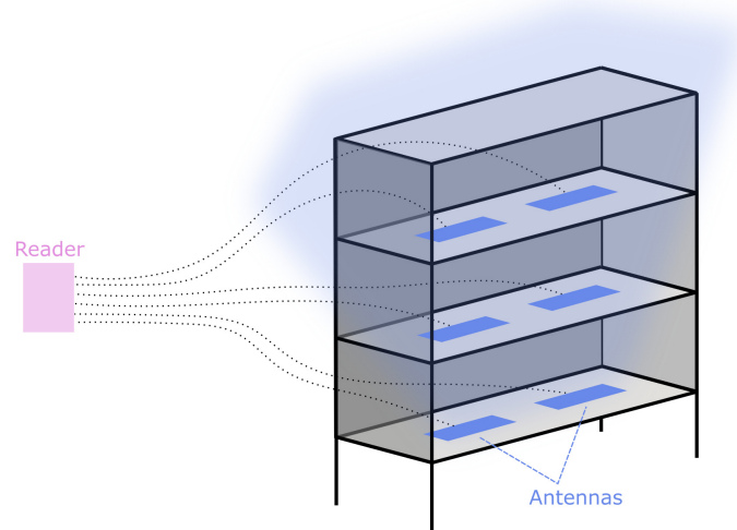
Figure 5.4: Arrangement with multiple compact antennas distributed in each shelf radiating upwards
