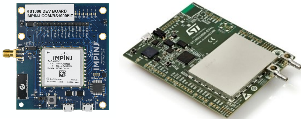
(a) Impinj RS1000 development kit (End-of-Life announced on September 4, 2020) (b) STMicroelectronics ST25RU3993 evaluation board ($306.25 at Digikey)
