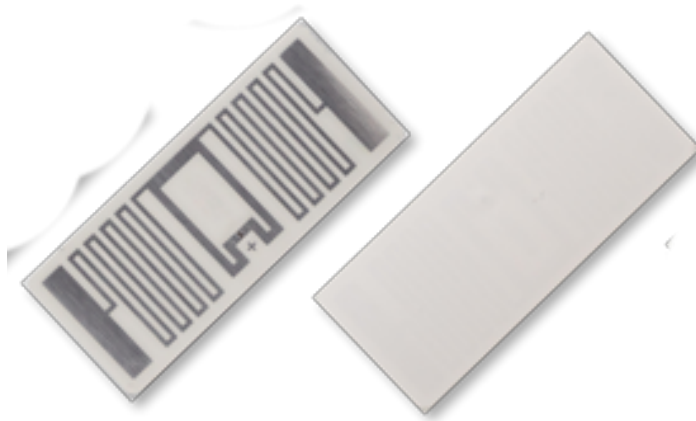
Figure 5.10: HID 6H2E43 92 × 28mm PET tag with 96 bit EPC [172]
