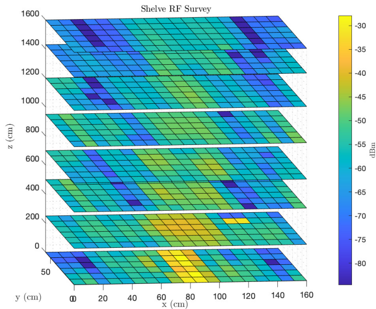
Figure 7.3: Shelf RF survey showing the RSSI values within the 20 \times 7 grid
