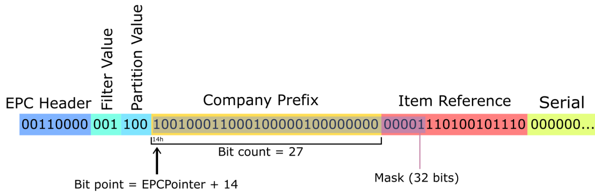
Figure 6.4: Illustration of company prefix C1G2 filtering parameter deduction
