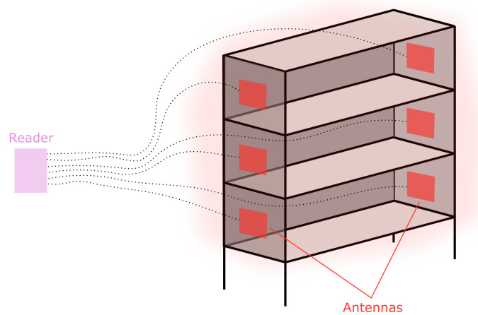
Figure 5.5: Arrangement with two antennas per shelf, one in each side of opposing laterals radiating inwards
