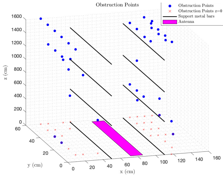
Figure 7.4: RF survey obstructions points shown in conjunction with support metal bars and antenna placement
