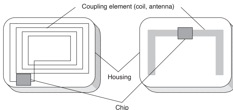
Figure 2.4: Components of a passive tag [14]
