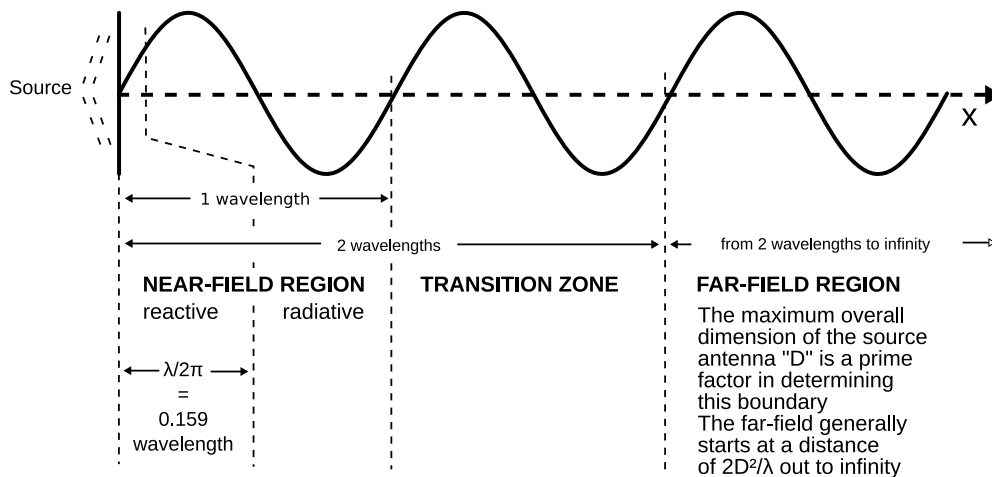
Figure 2.3: Fields for antennas equal to, or shorter than, one-half wavelength of the radiation they emit [20]
