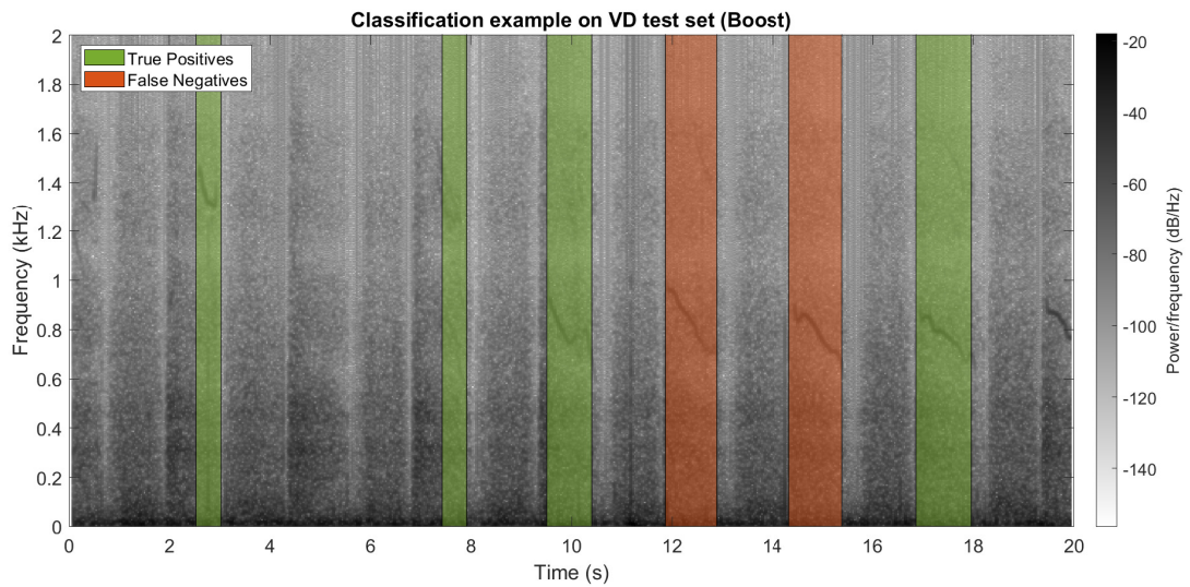
Fig. 4: Classification example VD (file: 133_3p4_Tc_mc_AKGC417L.wav)
