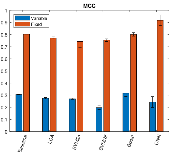
Fig. 2: MCC values for 10 runs in both experiments (mean and standard deviation).
