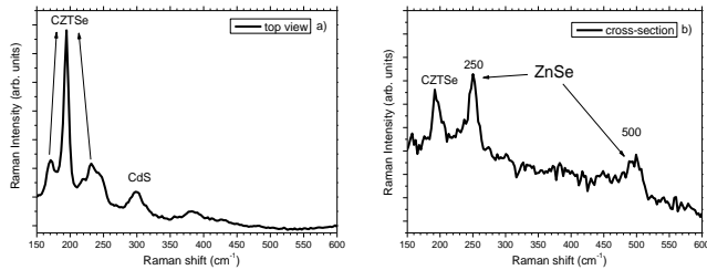
Figure 5: Raman scattering spectroscopy analysis of the a) surface and b) cross-section of a CZTSe sample. The surface measurement shows only the presence of CZTSe and CdS, whereas the cross-section reveals the appearance of ZnSe.
