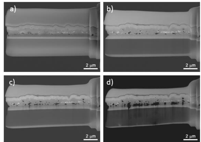
Figure 4: Evolution of the lamella with the thinning-down process at several acceleration voltage stages. a) and b) show the evolution during the 30 kV stage, c) after the 2 kV stage, and d) the final result after a 1 kV polishing stage.
