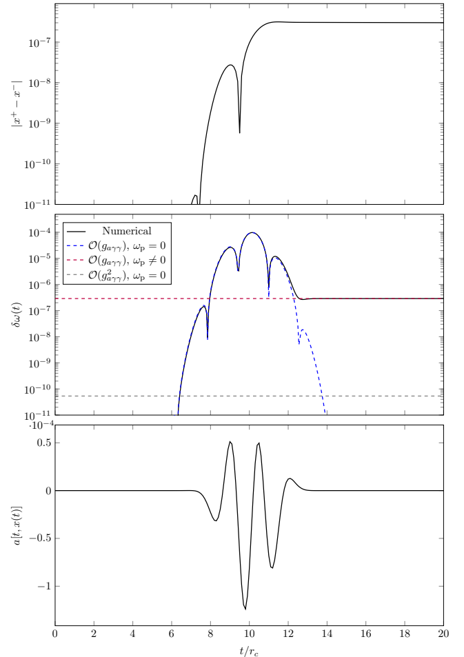
FIG. 1. Top panel. Relative position/time splitting between left-right polarised photons in the presence of plasma. Middle panel. Frequency shift for the left-polarised mode. We show the analytic results with and without plasma for comparison. The analytic results in the legend correspond to eq. (39) (blue-dashed) as well as the asymptotic frequency shifts from eqs. (36) and (37) shown as the dashed horizontal lines. Bottom panel. Axion profile evaluated along trajectory. We used the toy profile a = a_0 \sin(m_a t) e^{-x^2/r_c^2} with g_{a\gamma\gamma} a_0 = 10^{-4} , m_a r_c = 0.5 and k_0 r_c = 5 . The plasma density is \omega_p/k_0 = 0.08 and the frequency and position are given in units with r_c = 1 .
