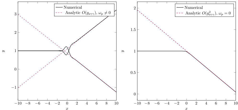
FIG. 3. Left panel. Refraction through an axion cloud of left/right modes (black lines) with plasma, compared to the asymptotic trajectory (red-dashed) predicted by eq. (46). The black lines show the rays (x(t), y(t)) given by solving the geodesic equations (18)-(20) numerically. The axes have been arbitrarily re-scaled for visibility. We chose an impact parameter b = r_c and a localized Gaussian axion profile, a = a_0 \sin(m_a t) \exp(-(x^2 + y^2)/r_c^2) , for illustration purposes. With g_{a\gamma\gamma} a_0 = 5 \times 10^{-6} and m_a r_c = 0.3 , k_0 r_c = 30 and a plasma mass \omega_p/|k_0| = 0.01 . Right panel. Refraction through an axion background without plasma, \omega_p = 0 , with comparison to the asymptotic trajectory (red-dashed) predicted by eq. (48). The other values are the same. Rays propagate from the left to the right of the plot in both cases.
