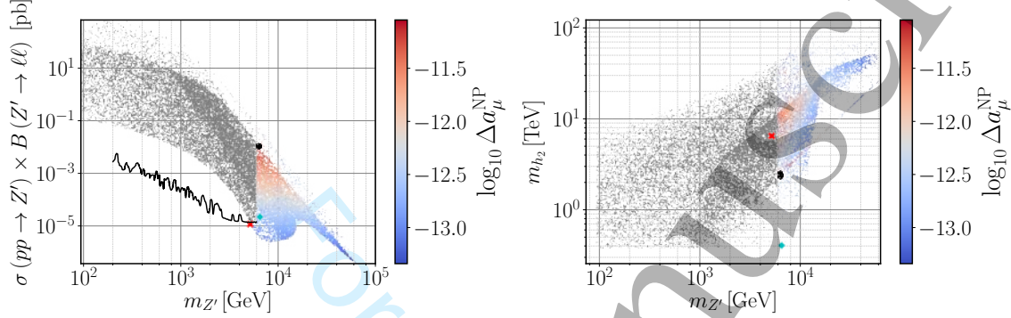
FIG. 3. Scatter plots showing the Z' Drell-Yan production cross section times the decay branching ratio into a pair of electrons and muons (left panel) and the new scalar mass m_{h_2} (right panel) as functions of m_{Z'} and the new physics (NP) contributions to the muon \Delta a_\mu anomaly. The solid line represents the current ATLAS expected limit on the production cross section times branching ratio into a pair of leptons at 95% C.L. taken from Ref. [53]. Coloured points have survived all theoretical and experimental constraints while grey points are excluded by direct Z' searches at the LHC. The six highlighted points in both panels denote the benchmark scenarios described in Tab. 4. These are represented by the red cross for the lightest Z' scenario (first row), cyan diamond for the lightest h_2 scenario (second row) and the black dots (last four rows).
