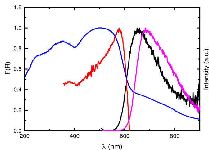
Fig. 8 Absorption (blue), fluorescence excitation (red, \lambda_{\text{exc}} = 650 nm) and emission spectra (black, \lambda_{\text{exc}} = 490 nm) of CR@CB[7](100). The emission spectrum of CR in the solid state is shown for comparison (magenta, \lambda_{\text{exc}} = 490 nm).
