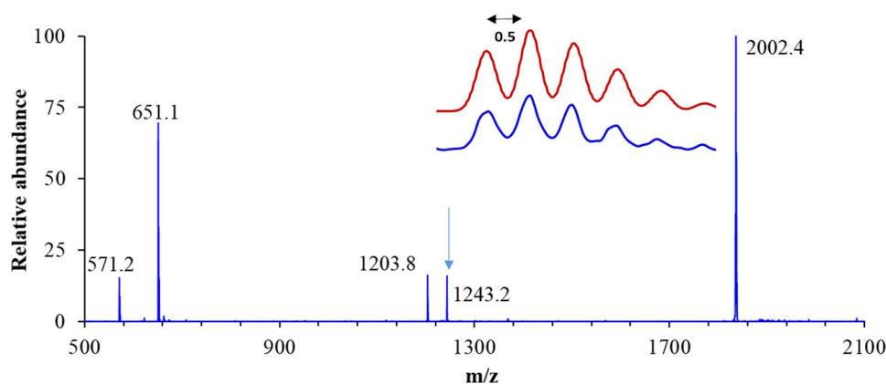
Fig. 4 Fragmentation spectrum ( MS^2 ) of m/z 1243.2. The arrow indicates the fragmented peak. The insert shows the experimental (blue) and simulated (red) isotope distributions.
