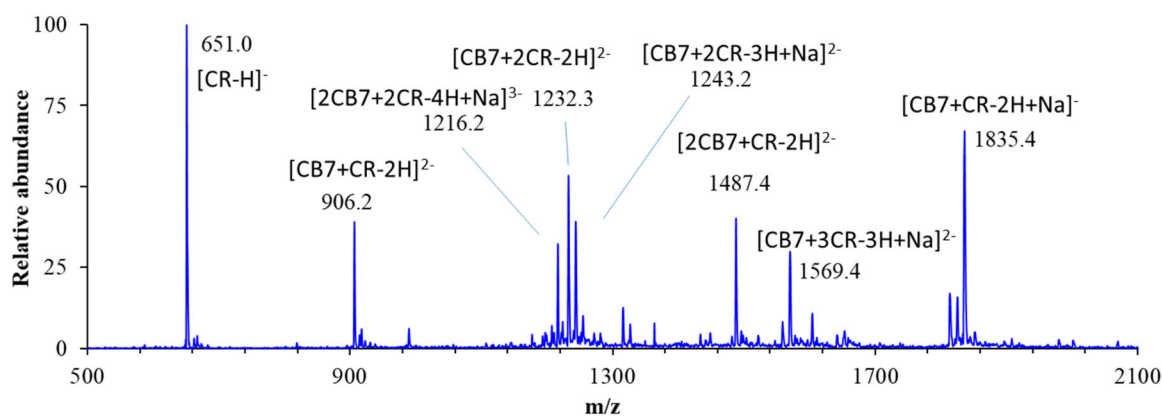
Fig. 3 Full scan spectrum of aqueous solutions of CR@CB[7] (50 \mu M : 50 \mu M) under negative ESI. The m/z values are of the first peak of the isotope series.
