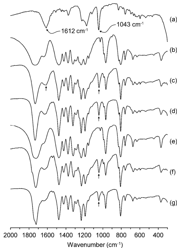
Fig. 5 FT-IR spectra in the range of 300-2000 cm -1 for (a) CR, (b) CB[7], (c) CR@CB[7](RT), (d) CR@CB[7](100), (e) CB[8], (f) CR@CB[8](RT), and (g) CR@CB[8](100). CR bands at 1043 and 1612 cm -1 are indicated with arrows.
