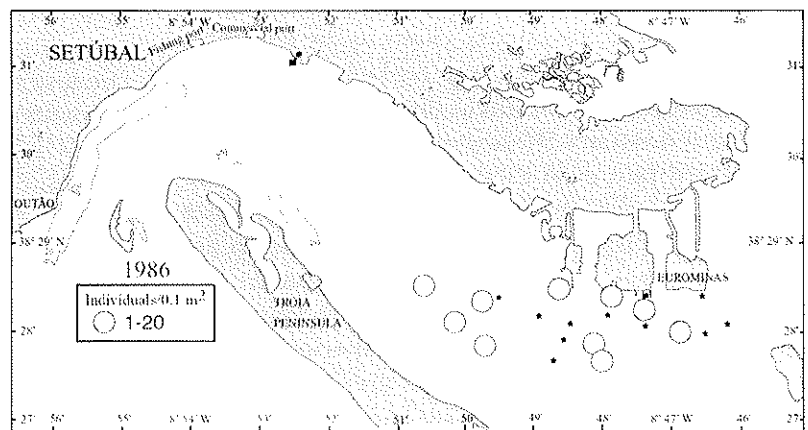
Figure 7. Abundance of Corbula gibba in 1986. ★: site where the species was absent
