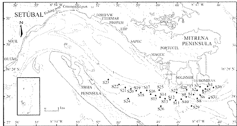
Figure 1. Location of sampling sites. Depth in metres. Intertidal areas are shown in light grey
