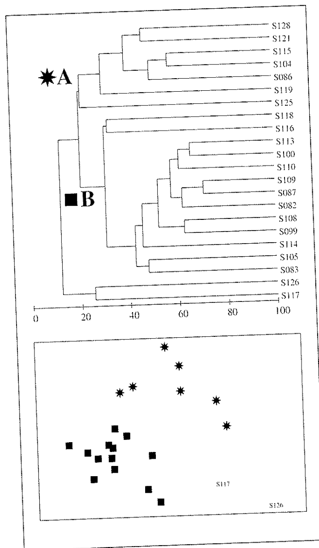
Figure 6. Classification ordination diagrams concerning 1986 biological data
