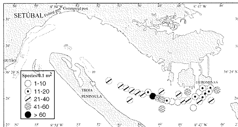
Figure 2. Spatial distribution of species richness
