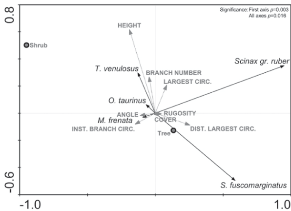
Fig. 1. RDA correlation biplot of species and microhabitat variables. Species are represented by black solid lines, microhabitat variables (MH) are represented by dotted grey lines and capitalized letters. Centroids from the variables “tree” and “shrub” of nominal MH “vegetation type” are represented as grey, filled circles.
