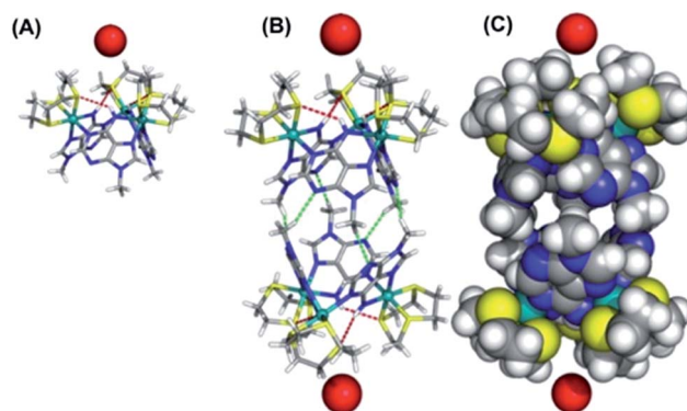
Fig. 2 (A) Details from the single crystal X-ray structure of [1](\text{Br})_3 showing the weak N–H⋯S hydrogen bonds (red dashed lines) within the of 1^{3+} unit. (B) Dimeric 'capsules' formed in the structure through C–H⋯N hydrogen bonds (green dashed lines) between facing bowls. (C) CPK model of capsules showing axial entrances occupied by bromide anions and equatorial 'gates' locked by the steric bulk of N -methyl groups of 9MA ligands. The following atomic colour scheme was used: carbons in grey, hydrogens in white, sulfurs in yellow, nitrogens in blue, ruthenium centres in teal and bromide anions in red.
