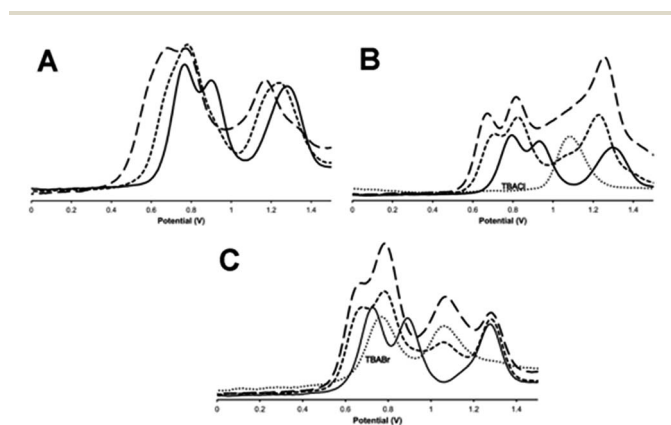
Fig. 6 Square wave voltammograms, SWVs, for the oxidations of 1^{3+} on the addition of (A) TBAF; (B) TBACl; (C) TBABr. Key: (—) untreated 1^{3+} , (---) +1 equivalent of guest, (···) +3 equivalents of guest. In (B) and (C) (···) SWV of TBACl and TBABr respectively in identical conditions (vs. Ag/AgCl solvent: 0.1 M TBAPF 6 in acetonitrile).
