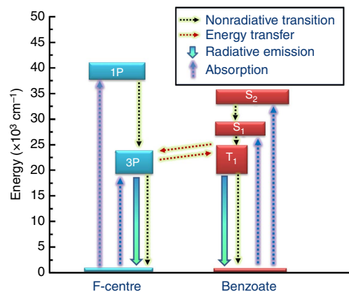
Figure 3 | Excitation and relaxation pathways diagram. Energy levels and possible relaxation pathways in the boehmite hybrid nanoparticles (B1). The energy position of the singlet ( S_1 and S_2 ) and triplet ( T_1 ) states relative to the benzoate were extracted from the previous analyses of the excitation spectrum and from the zero phonon line of the vibrational progression observed in the emission spectrum. The singlet (1P) and triplet (3P) energy values related to the F-centre correspond to the maximum intensity peak position of the components in the excitation and emission spectra of the W1 model nanoparticles, respectively. In all the cases, the width of the levels accounts for the FWHM of the bands in the emission and excitation spectra.
