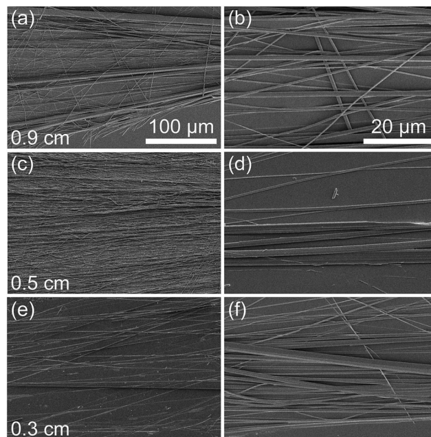
Fig. 3 SEM images of aligned heated PNTs ( 2 \text{ mg ml}^{-1} FF) prepared using (a and b) 0.9 cm, (c and d) 0.5 cm, and (e and f) 0.3 cm mask openings.
