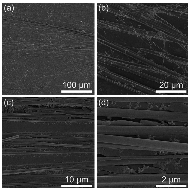
Fig. 4 (a and b) SEM images of PNTs coated with Ag NPs. (c and d) SEM images of aligned Ag NP-coated PNTs after adding TMPyP.
