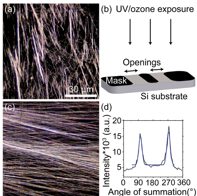
Fig. 1 (a) Optical image of randomly oriented PNTs. (b) Schematic of the mask used to achieve alignment. (c) Optical image of aligned PNTs. (d) Radial summation of the FFT intensity versus angle showing Gaussian fits (blue line) used to determine the FWHM, i.e. , the degree of alignment.
