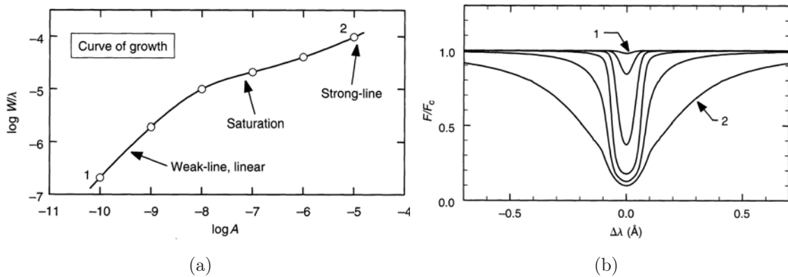
Figure 2.2: a) Typical curve of growth from a model photosphere: log-log plot of the reduced EW ( W/\lambda ) with abundance ( A ).; b) Line profile change with chemical abundance of the absorbing species. The dots in (a) correspond to the different lines in (b).
