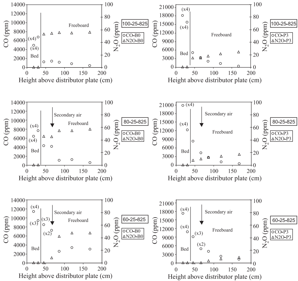
Fig. 5. N 2 O and CO axial concentration profiles during bituminous (B0) and anthracite (P3) coal combustion (100%, 80% and 60% primary air; 25% excess air; 825 °C bed temperature).
