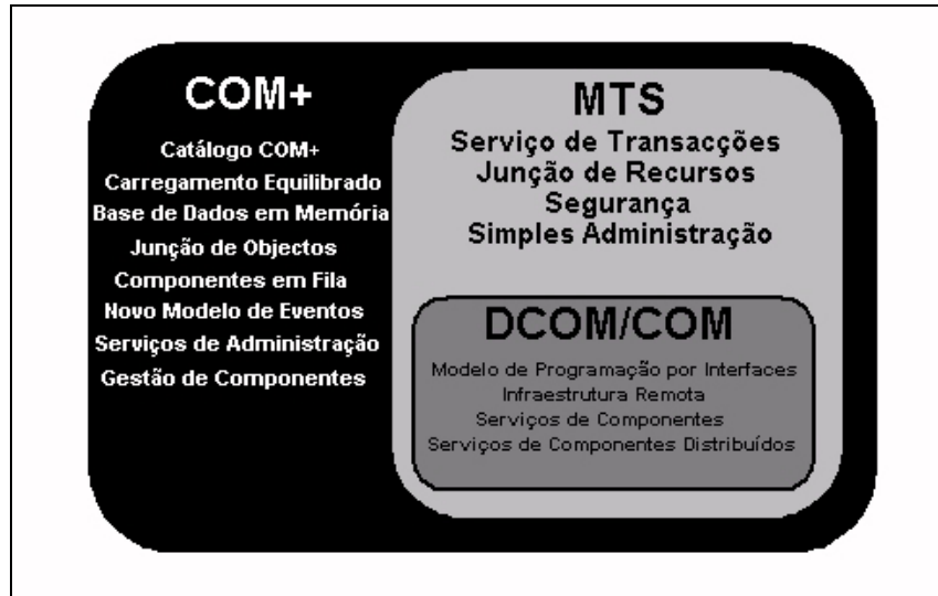
Figura 52 - COM+ [Armstrong - 1999].
